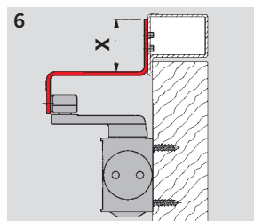
6 Parallel arm bracket with upstand (*upstand 35 or 60 mm)
