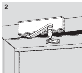
2 Frame installation
